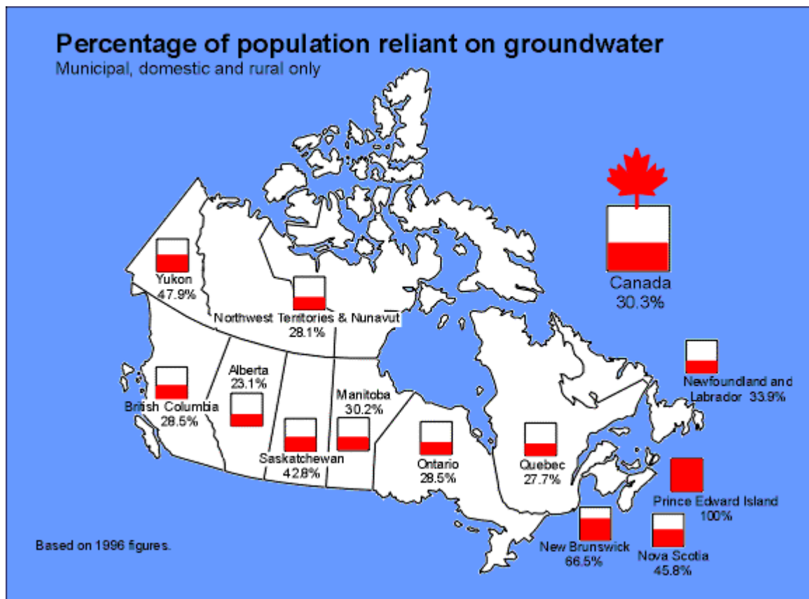
Figure 6.3 Percentage of Canadian Population Reliant on Groundwater
